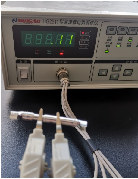
图片 3 LEADER 插套 & T4 插针 LEADER socket & T4 pin
