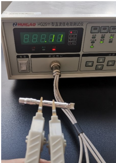
图片 5 LEADER 插套 & MC4 插针 LEADER socket & MC4 pin
