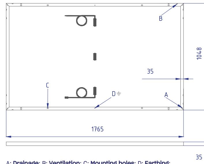
A: Drainage; B: Ventilation; C: Mounting holes; D: Earthing;
